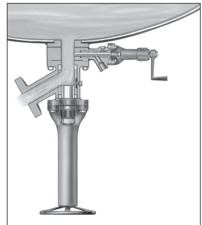
Fig. 3 - Drain Valve Fully Open
