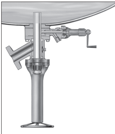
Fig. 1 - Drain Valve Fully Closed
